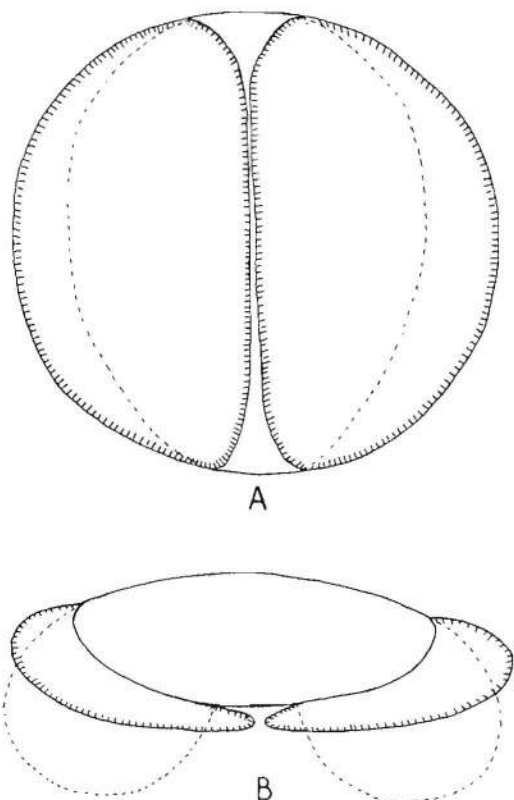
TEXT-FIG. 14 — Organization of Sulcatisporites (Leschik) emend. A, polar view. B, meridional sections of flattened and unflattened specimens.
