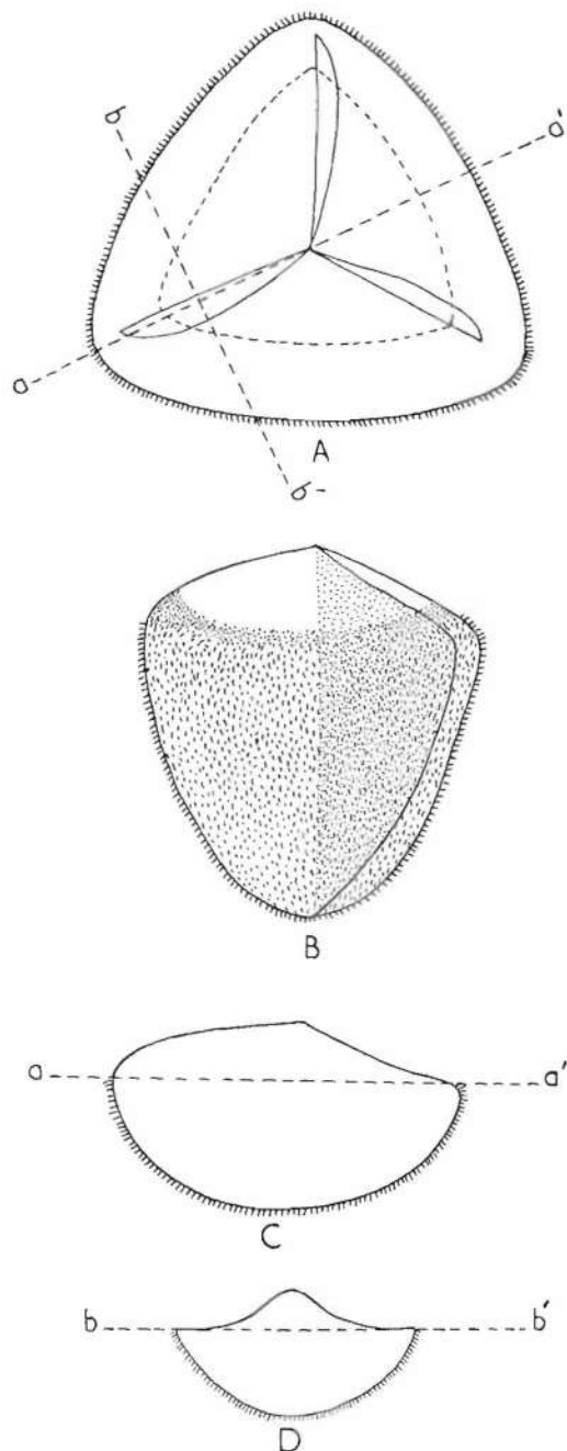
TEXT-FIG. 4 — Organization of Microbaculispora gen. nov. A, polar view. B, meridional view. C, meridional section along a, a' in A. D, meridional section along b, b' in A.
