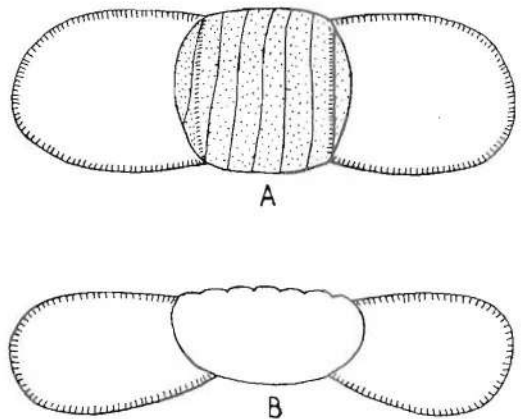
TEXT-FIG. 13 — Organization of Striapollenites gen. nov. A, polar view. B, meridional section.
