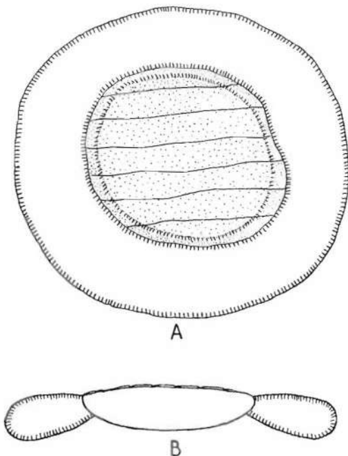
TEXT-FIG. 8 — Organization of Striomonosaccites gen. nov. A, polar view. B, meridional section.
