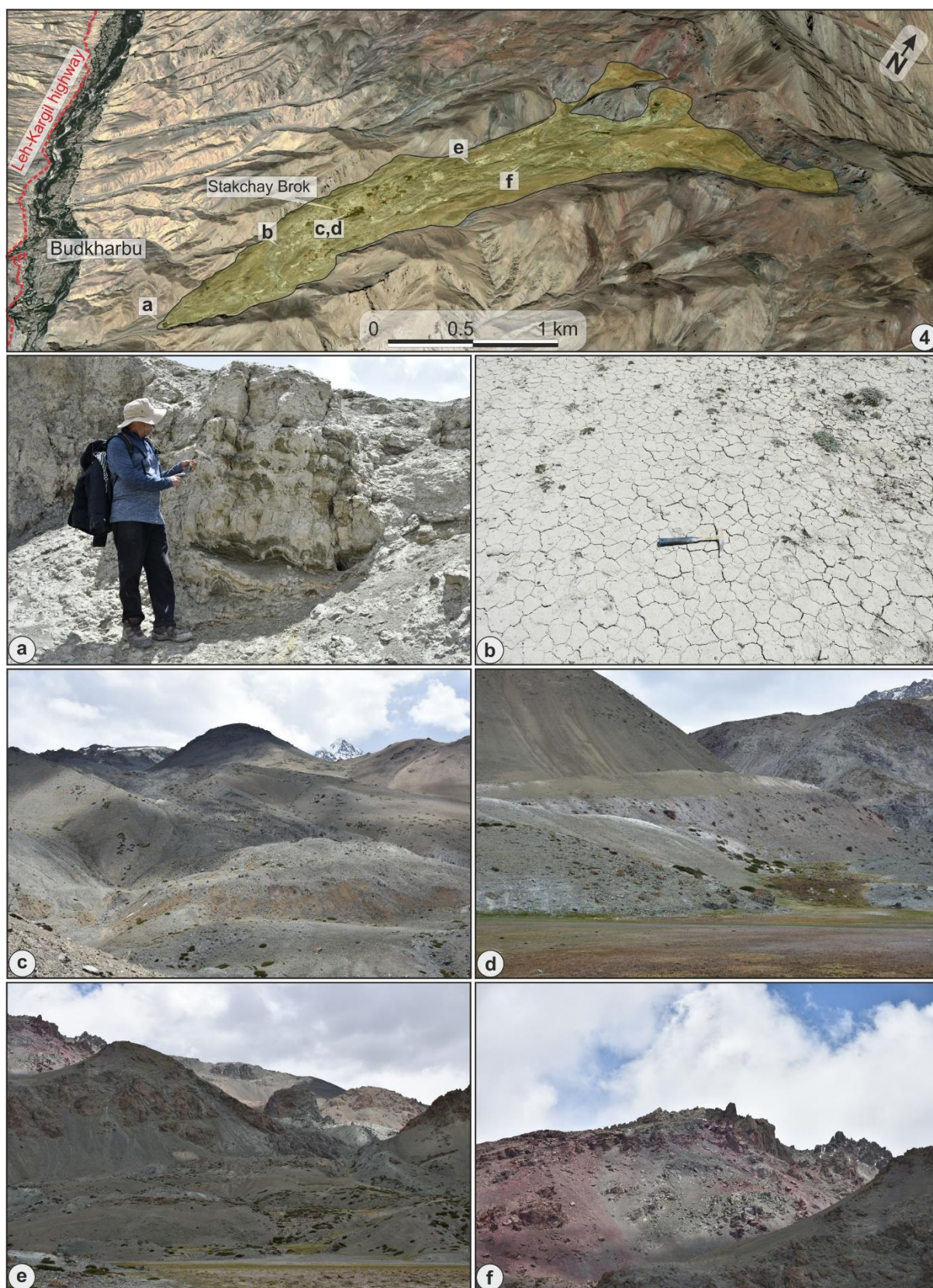
Fig. 12. Google Earth Pro image showing the rock glacier boundary (highlighted area) and its surroundings. The location of different field photographs is also marked on the image (Zone-II) showing (a) a succession of relict lake sediments that is a represent of sedimentation in some
