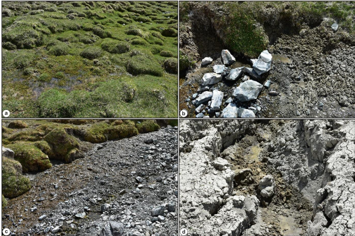
Fig. 7. Field photographs showing the evidences of thawing of the RG interstitial ice at various locations of zone II and III on the SBRG.
