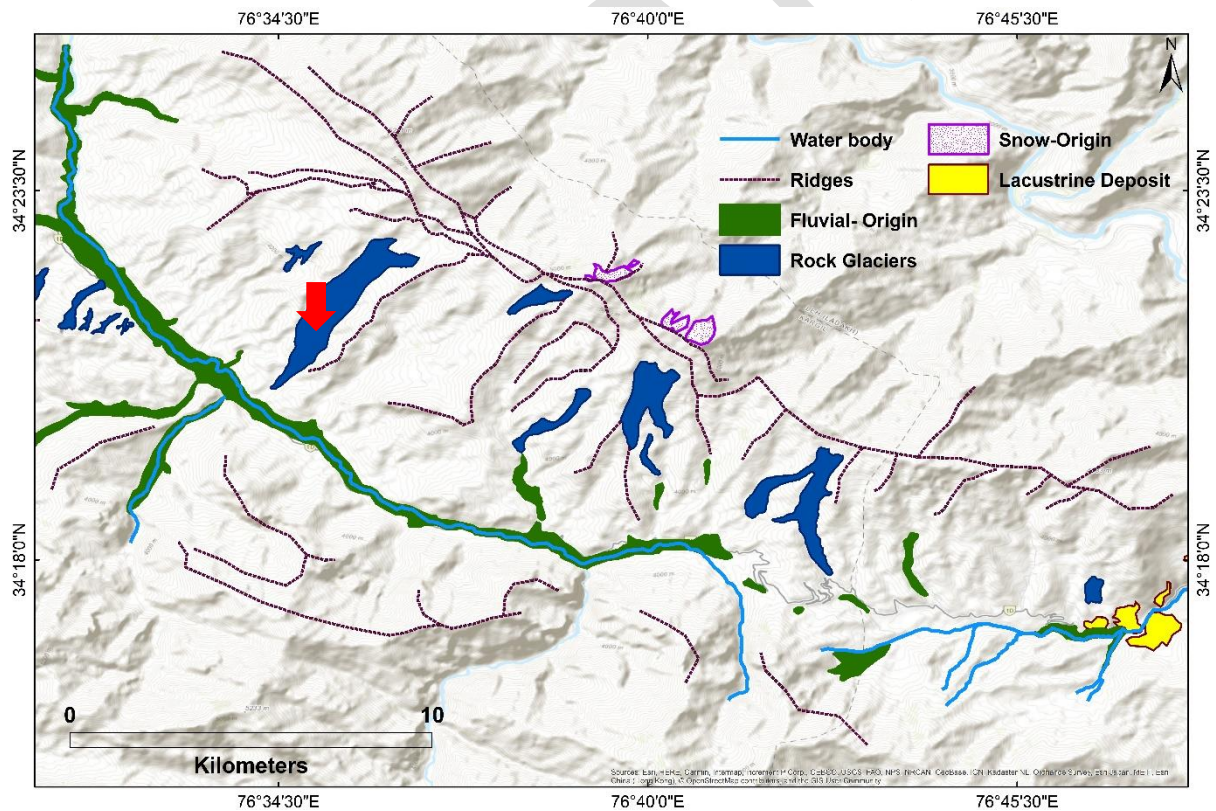
Fig. 2. Location and a generalized geomorphological map showing Stokchey Brok village (marked by red arrow) near Budhkharbu on the base map of ArcGIS.
