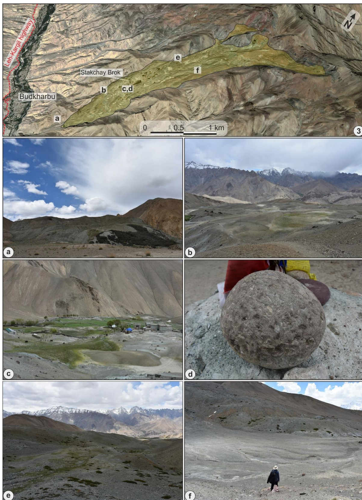
Fig. 9. Google Earth Pro image showing the rock glacier boundary (highlighted area) and its surroundings. The location of different field photographs is also marked on the image showing (a) the frontal lobe of the rock glacier, the green patch is the bushy vegetation growing along
