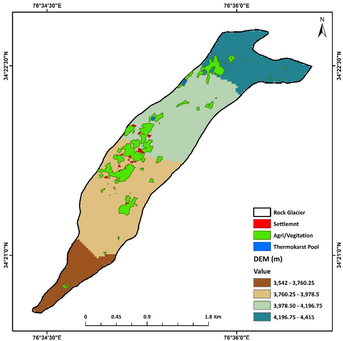
Fig. 8: Four elevation zones (I-IV) of the SBRG.
